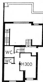
PIANO TERRA
